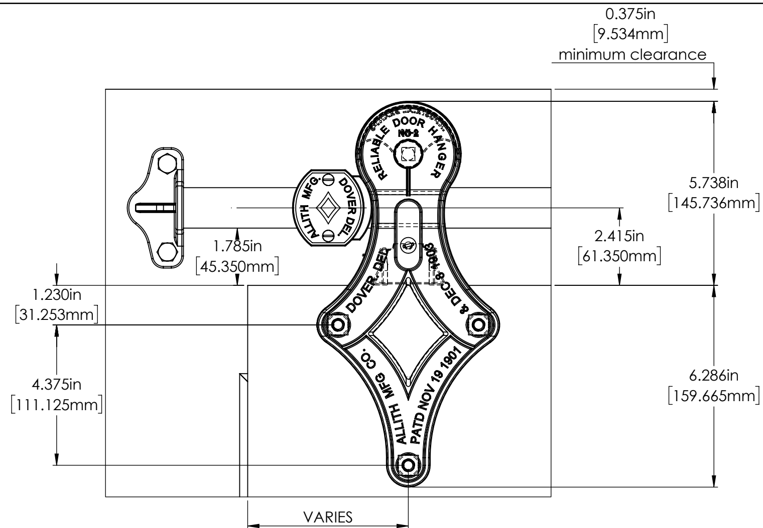
DETAIL C SCALE 1 : 3
