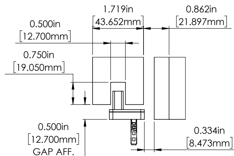
DETAIL E SCALE 1 : 2
