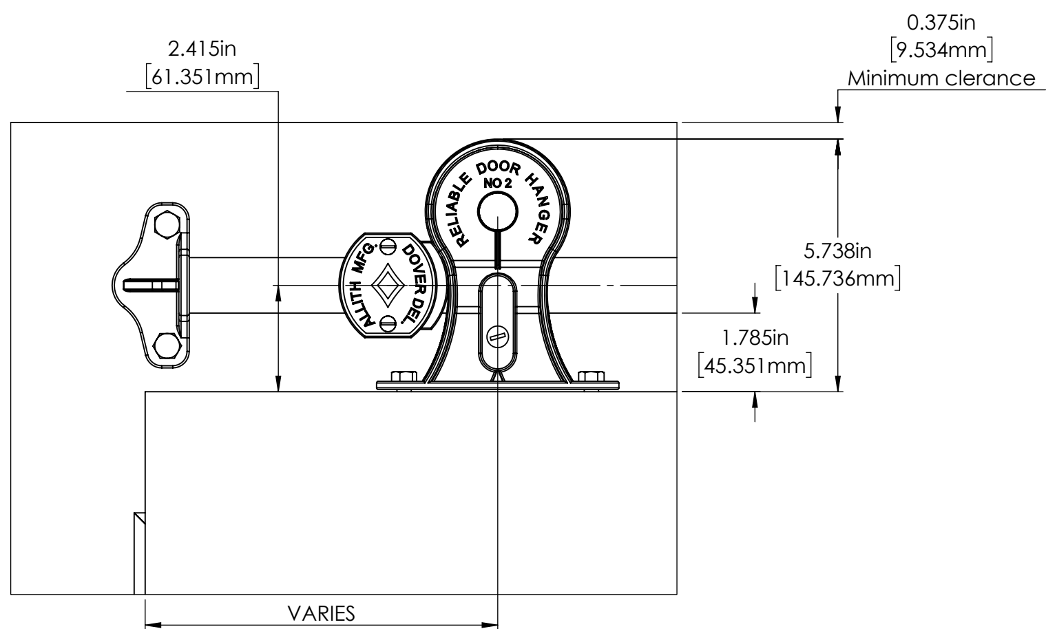
DETAIL C SCALE 1 : 3
